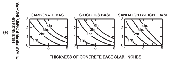
FIGURE 721.2.2.3(2) FIRE-RESISTANCE RATINGS FOR CONCRETE
