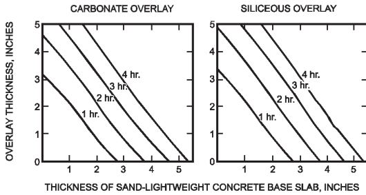
FIGURE 721.2.2.2 FIRE-RESISTANCE RATINGS FOR TWO-COURSE
