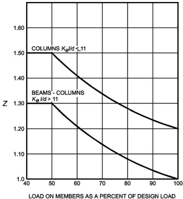
FIGURE 721.6.3(1) LOAD FIGURE
